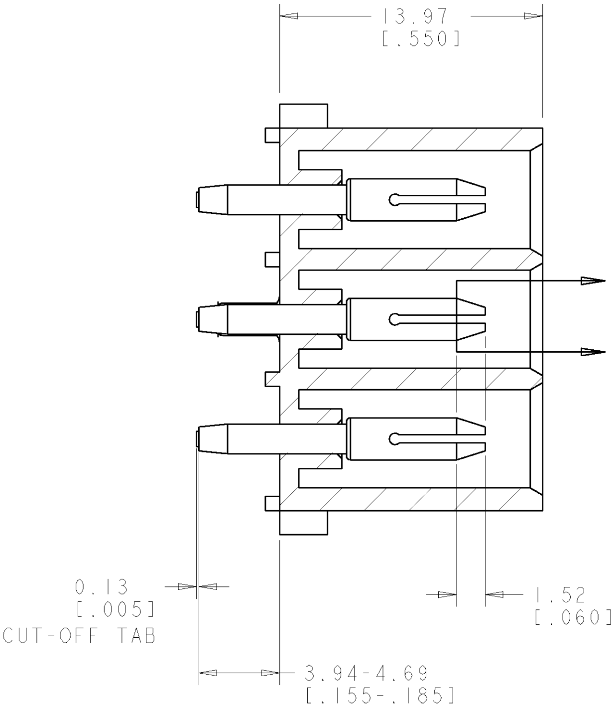
SECTION B-B
